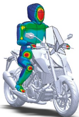
Wind pressure with Windshield Naked New Generation Puig.
