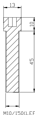
M10/150(LEFT THREAD)
