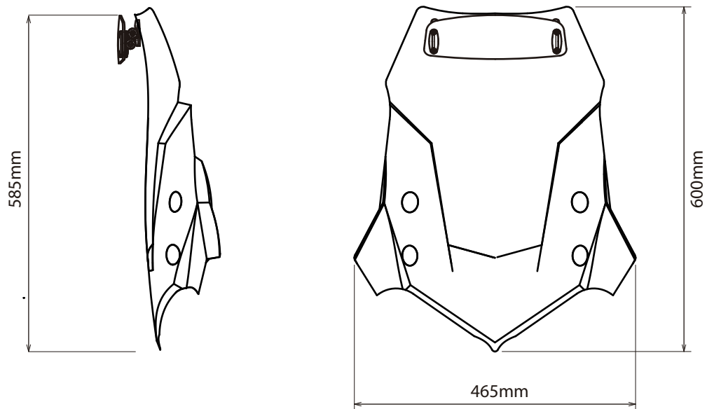
TOURING SCREEN WITH VISOR AT UPPER POSITION
