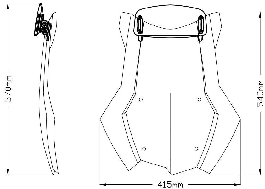
TOURING SCREEN WITH VISOR AT LOWER POSITION
