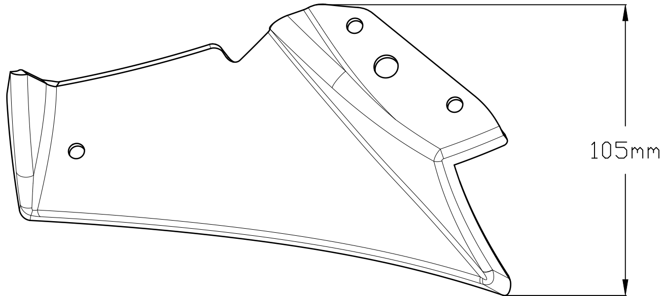
RIGHT DEFLECTOR
